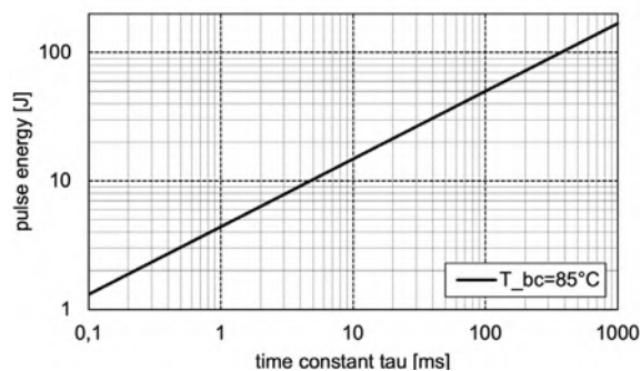
Typical Pulse Load Capability
