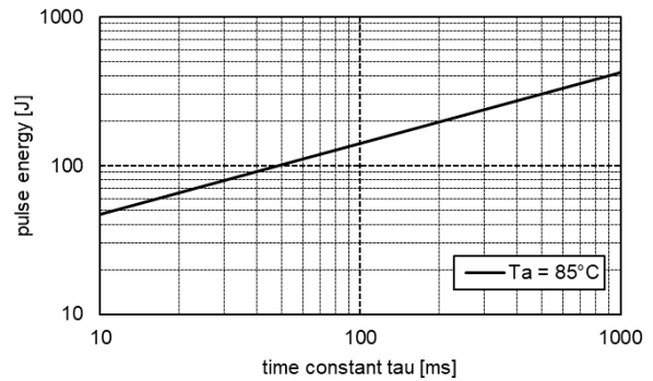
Typical Pulse Load Capability
