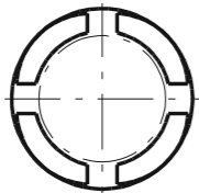
4 tilting pads
